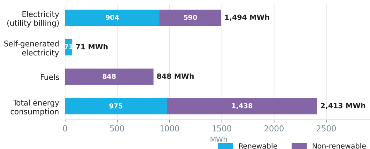
Figure 1. Energy consumption by source, renewable vs. non-renewable (MWh), 2025.
